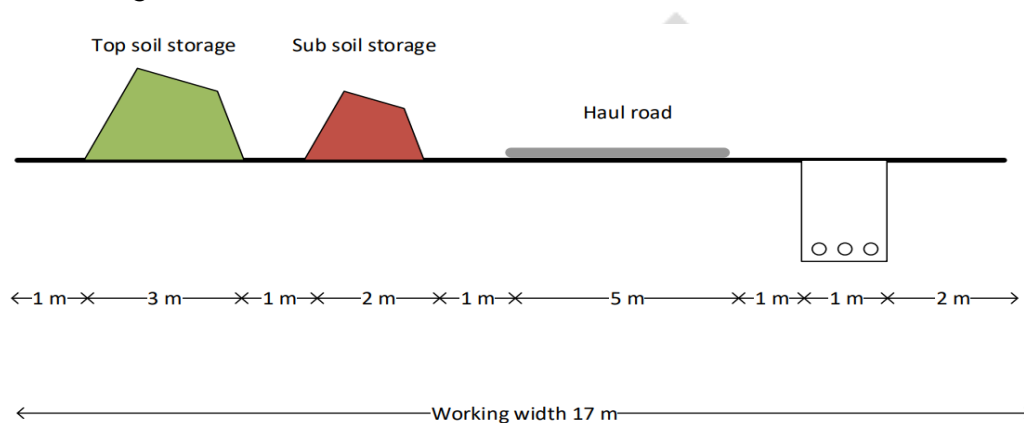
Figure 4.6: Working Corridor for Cables (source: WSP | not to scale)
