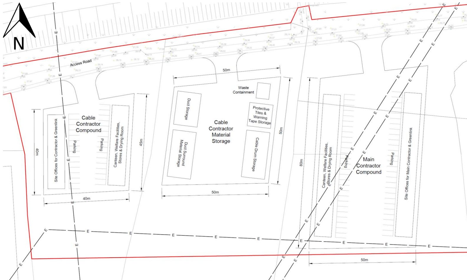
Figure 4.5 Contractors' Compounds at Great Island | not to scale
