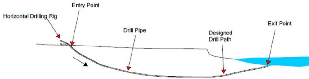
Figure 4.8 Typical HDD Installation at a Typical Landfall | not to scale
