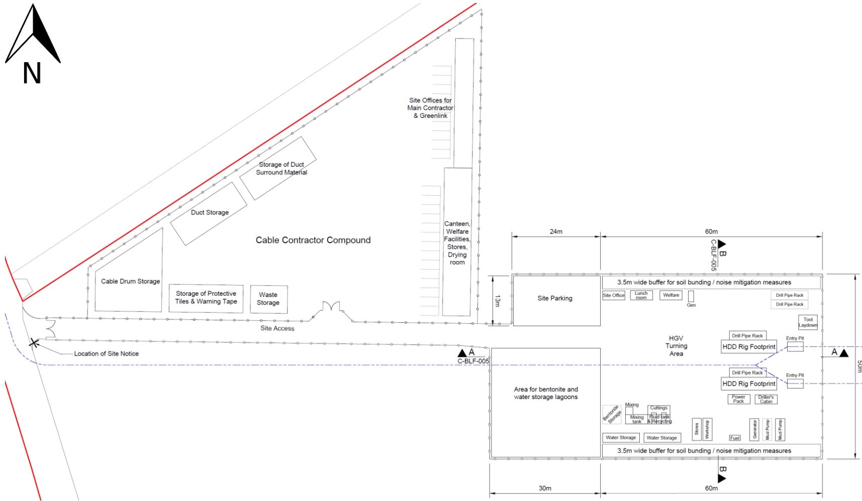
Figure 4.2 Contractors' Compounds near Baginbun Beach | not to scale [cable route shown in blue]
